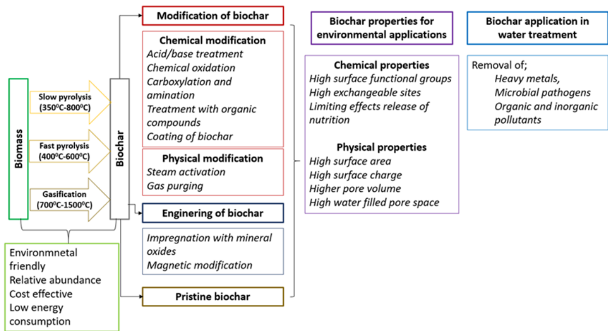
Figure 1. Strategic schematic diagram for biochar production, modification/engineering, characteristics, and water treatment applications
